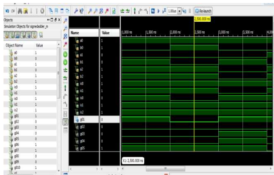
Fig 3: simulation result of single digit adder cell
