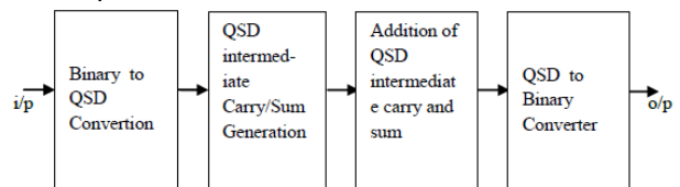
Fig1. General Block Diagram of QSD Addition
