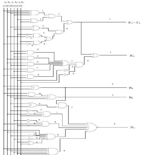
Figure 1: Data Flow of single digit QSD adder cell.
