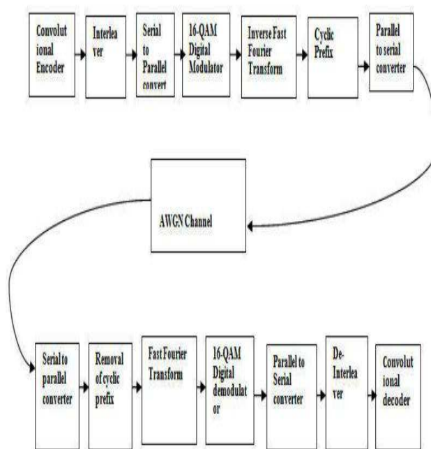
Figure 1 .Block diagram of convolution coded OFDM
