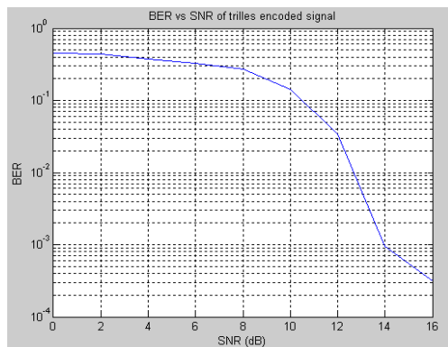
Figure 4. performance of CCOFDM over AWGN channel.
