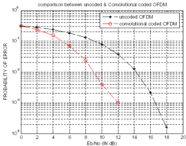
Figure 3. Performance analysis between uncoded and convolution coded OFDM system
